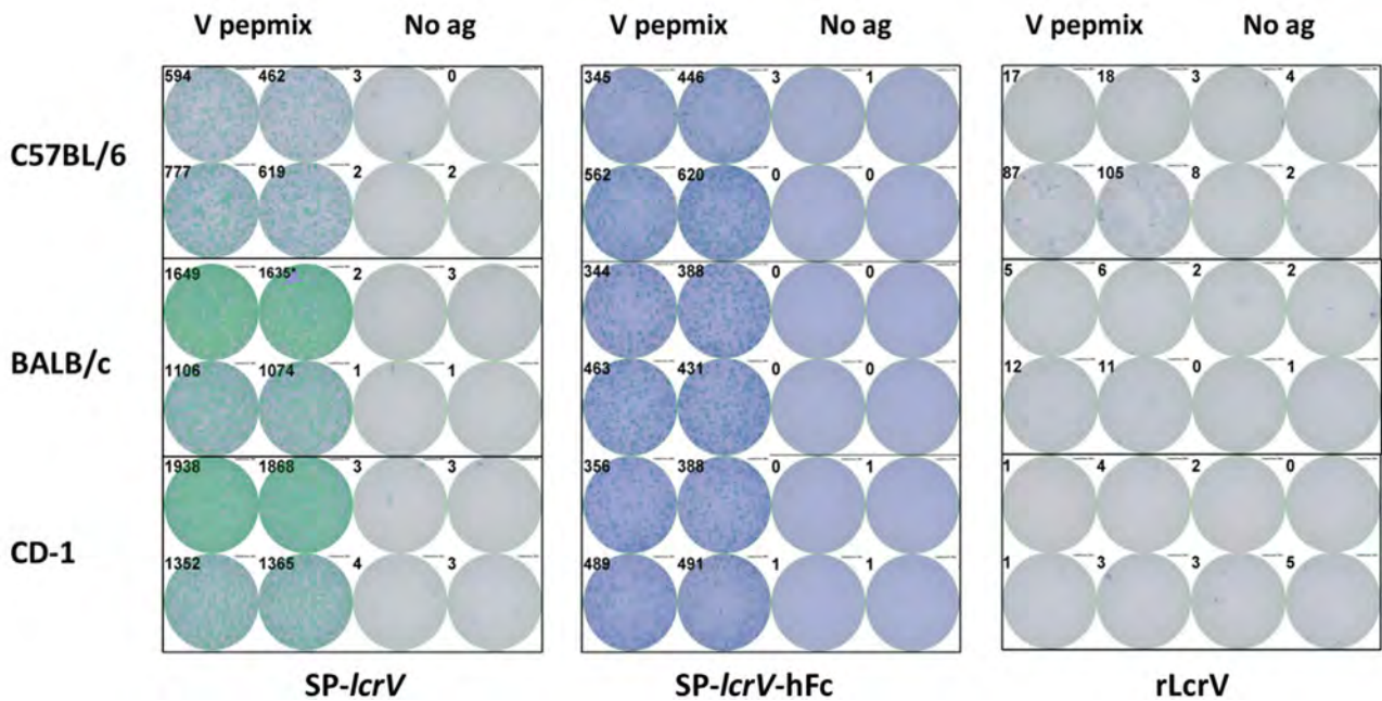
Figure 4. Induction of antigen-specific cellular immunity by LcrV mRNA vaccine. Spleens were collected from SP-IcrV, SP-IcrV-hFc or rLcrV vaccinated animals ( n = 3-4 ) 14 days after the last vaccine administration. Antigen-specific cellular response was determined by ELISpot assay by quantification of IFN- \gamma secreting cells A). Panel B shows representative wells from the ELISpot assay, used for quantification. Statistical analysis was performed using a two-way ANOVA with Bonferroni's multiple comparisons test (* p < 0.05 , ** p < 0.01 ).
