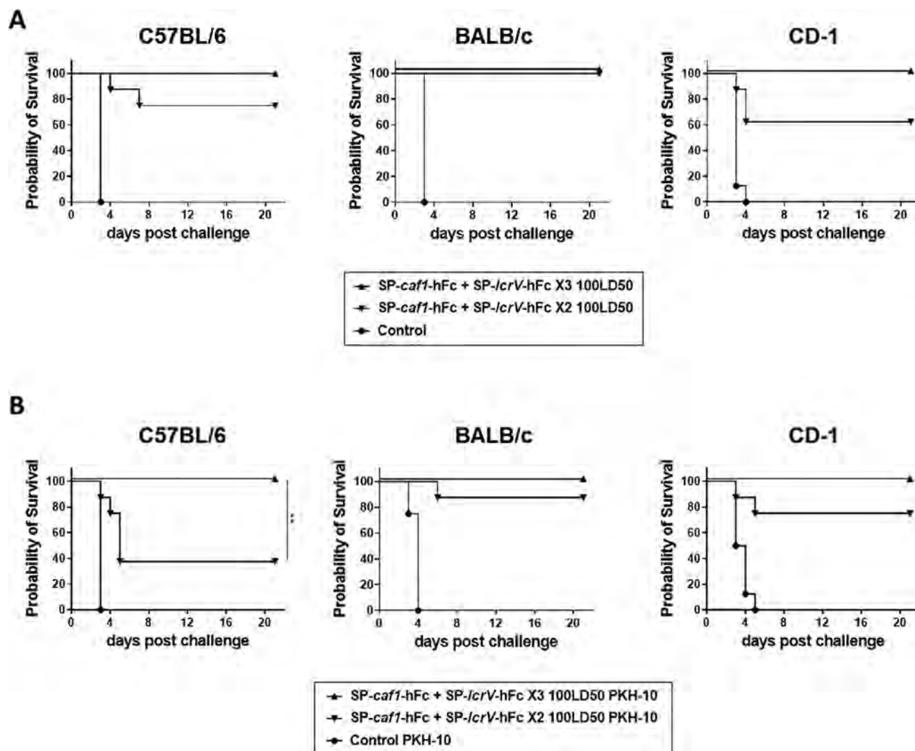
Figure 6. Protective efficacy of bivalent F1 + LcrV mRNA-LNPs against high dose intranasal challenges with two different Y. pestis biovars. C57BL/6, BALB/c, and CD-1 mice ( n = 8) were vaccinated intramuscularly with 2 or 3 doses of a combination of SP- lcrV -hFc and SP- caf1 -hFc (5µg each). Two weeks after the last vaccination (day 42), animals were subjected to high dose (100LD 50 ) Kimberley53 (A) or PKH-10 (B) challenges and monitored for survival. Statistical analysis was performed using log-rank (Mantel-Cox) test (for survival plot), (** p < 0.01).
