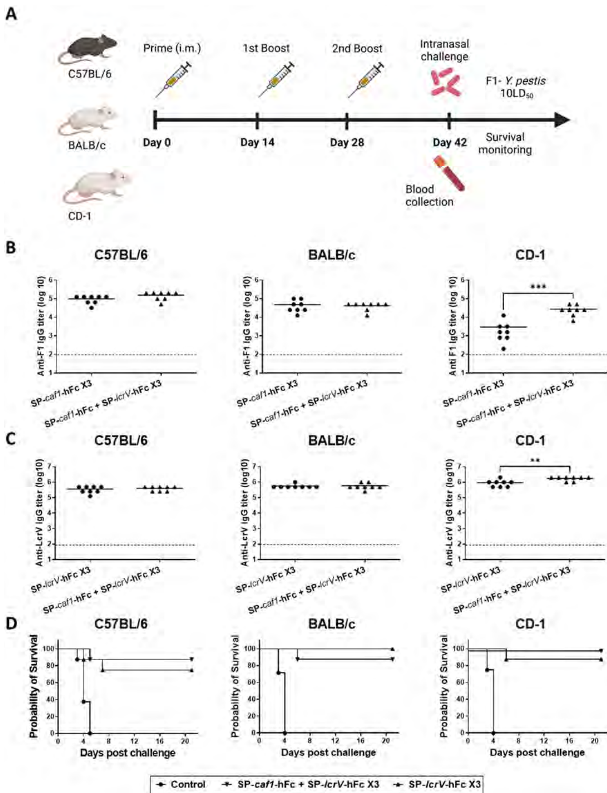
Figure 7. Immunogenicity and protective efficacy of bivalent F1 + LcrV mRNA-LNPs against the unencapsulated F1 Y. pestis strain. A) Schematic representation of vaccination regimen. C57BL/6, BALB/c and CD-1 mice ( n = 8 ) were vaccinated intramuscularly with either SP-lcrV-hFc ( 5\mu\text{g} ) or a combination of SP-lcrV-hFc and SP-caf1-hFc ( 5\mu\text{g} each) thrice (days 0, 14, 28). Blood samples were collected 14 days before the challenge, and serum samples were assayed for anti-F1 (B) and anti-LcrV (C) IgG antibodies by ELISA. Two weeks after the last vaccination (day 42), animals were subjected to
