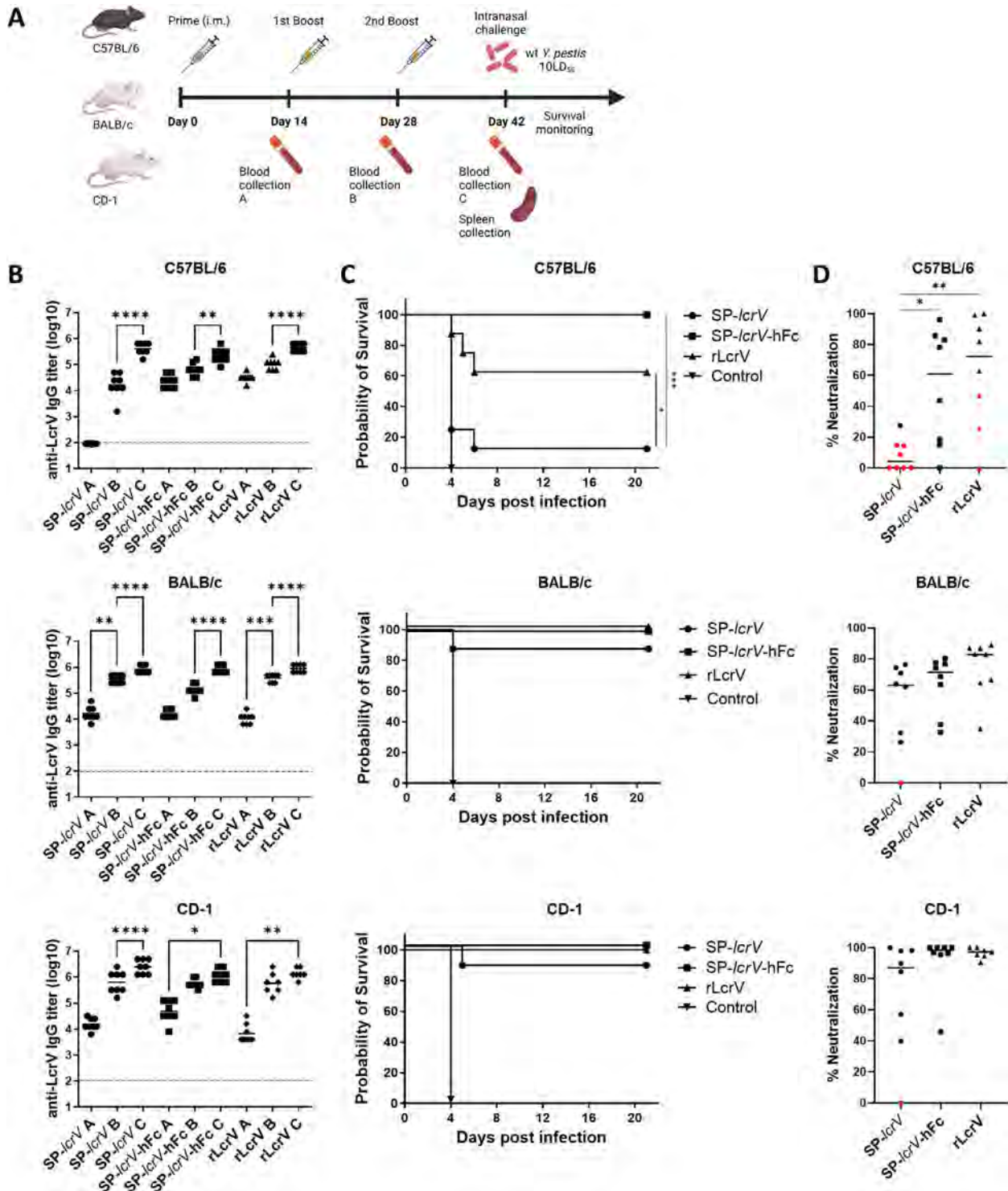
Figure 2. Immunogenicity and protective efficacy of LcrV against pneumonic Y. pestis in different mouse strains. A) Schematic representation of vaccination regimen. C57BL/6, BALB/c and CD-1 mice ( n = 8 / strain) were vaccinated intramuscularly with either SP- LcrV (5 μg), SP- LcrV -hFc (5 μg) or rLcrV (80 μg) at days 0, 14 and 28. Blood samples were collected before each booster dose (denoted as A, B, and C), and serum samples were assayed for anti-LcrV antibodies by ELISA. B) Two weeks after the last vaccination (day 42), animals were subjected to a lethal (10LD 50 ) intranasal challenge and monitored for survival. C) Sera from vaccinated mice were tested for cytotoxicity neutralization (% neutralization). Surviving animals are represented by black symbols and non-surviving animals are represented by red symbols. Mean % neutralization is indicated by horizontal black lines. Statistical analysis was performed using a one-way ANOVA with Tukey's multiple comparisons test (for immune responses and neutralization assay) or log-rank (Mantel-Cox) test (for survival plot), (* p < 0.05 , ** p < 0.01 , *** p < 0.001 , and **** p < 0.0001 ). Dashed line indicates limit of detection for ELISA. The schematic for panel 2A was created with Biorender.
