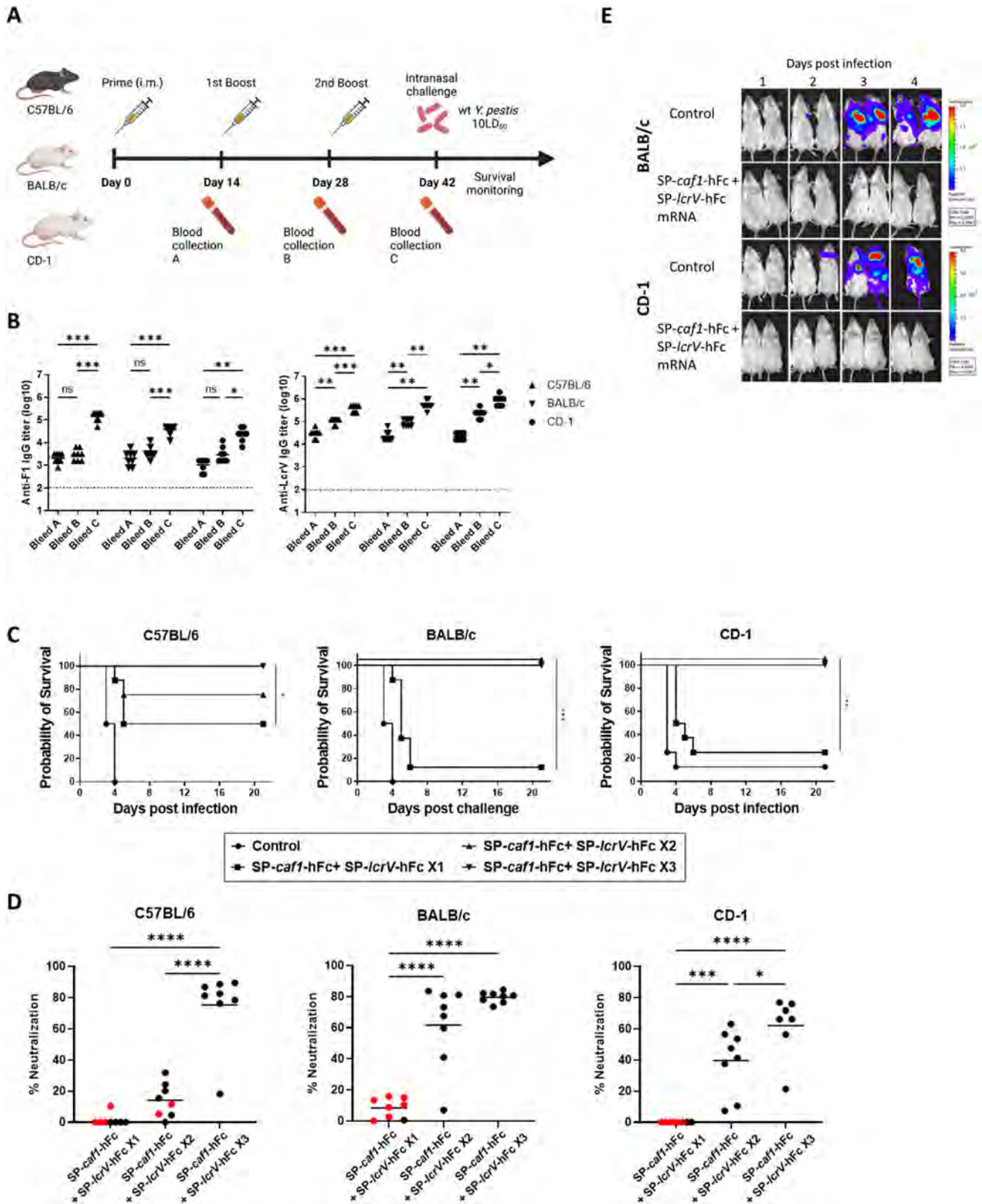
Figure 5. Immunogenicity and protective efficacy of bivalent F1 + LcrV mRNA-LNPs against pneumonic Y. pestis . A) Schematic representation of vaccination regimen. C57BL/6, BALB/c and CD-1 mice ( n = 8 ) were vaccinated intramuscularly with a combination of SP-lcrV-hFc and SP-caf1-hFc (5 \mu g each) once (day 28), twice (days 14, 28) or thrice (days 0, 14, 28). Blood samples were collected before each booster dose (A/B/C), and serum samples were assayed for anti-LcrV and anti-F1 IgG antibodies by ELISA (B). Two weeks after the last vaccination (day 42), animals were subjected to a lethal
