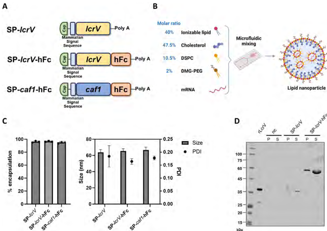
Figure 1. Design and synthesis of mRNA-LNPs used in the study, physicochemical characteristics and in vitro expression. A) Schematic representation of mRNA constructs utilized in the study. Elements include: Cap (Cap), signal peptide (SP), lcrV gene sequence ( lcrV ), caf1 gene sequence ( caf1 ), human Fc (hFc), poly adenylation (poly A). B) Schematic of mRNA-LNP formulation (see materials and methods section for more detail). C) Physicochemical characterization of mRNA-LNPs used in this study, showing average RNA encapsulation efficiency (left panel) and particle size and poly dispersity index (PDI, right panel). D) Western blot analysis of LcrV expression in HeLa cells transfected with the indicated mRNA constructs for 48 h. Recombinant LcrV served as size control. Protein expression was evaluated in both cell pellet (P) and supernatant (S). nc = negative control (untransfected cells). The schematic for panel 1B was created with Biorender.
