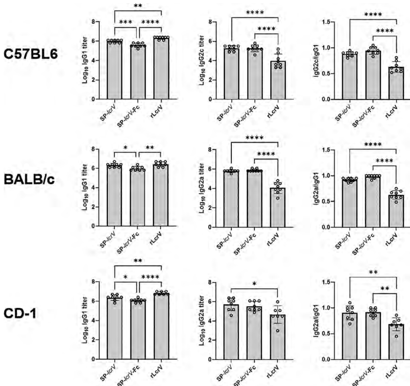
Figure 3. Induction of anti-LcrV IgG subclasses by mRNA or recombinant protein vaccine. Sera from BALB/c, CD-1 and C57BL/6 mice immunized thrice ( n = 8 ) with either SP-lcrV ( 5\mu\text{g} ), SP-lcrV-hFc ( 5\mu\text{g} ) or rLcrV ( 80\mu\text{g} ) were set to detect subclasses of anti-LcrV specific IgGs. Statistical analysis was performed using a one-way ANOVA with Tukey's multiple comparisons test ( *p < 0.05 , **p < 0.01 , ***p < 0.001 , and ****p < 0.0001 ).
